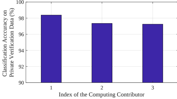
Fig. 10. Accuracy obtained by each computing contributor by using their local verification data.
