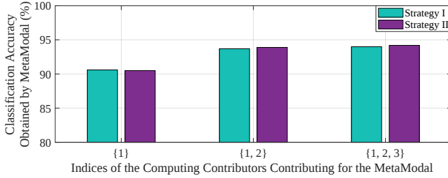
Fig. 11. Comparison of average classification accuracy obtained by MetaModal using strategies I and II versus the indices of the computing contributors contributing to the MetaModal.
